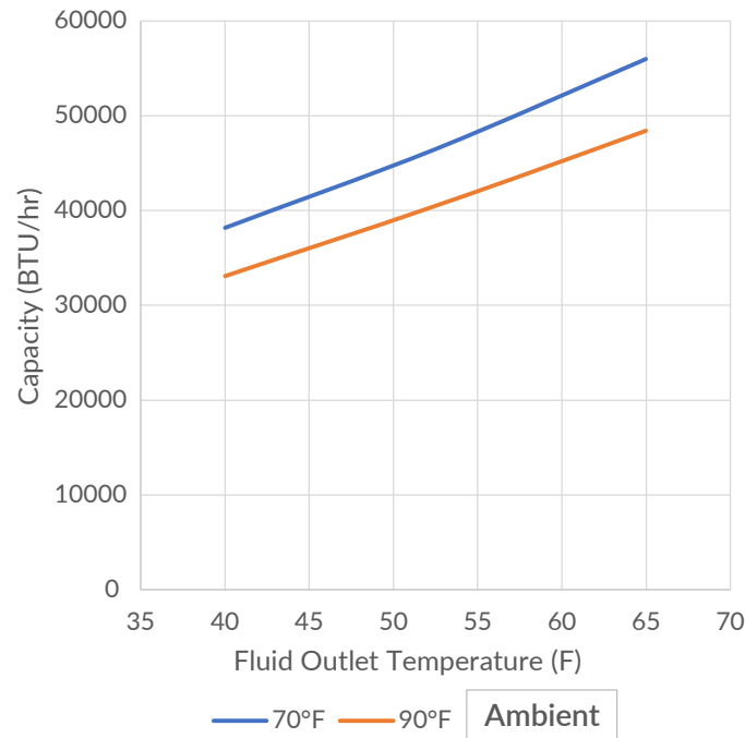
COOLING CAPACITY
